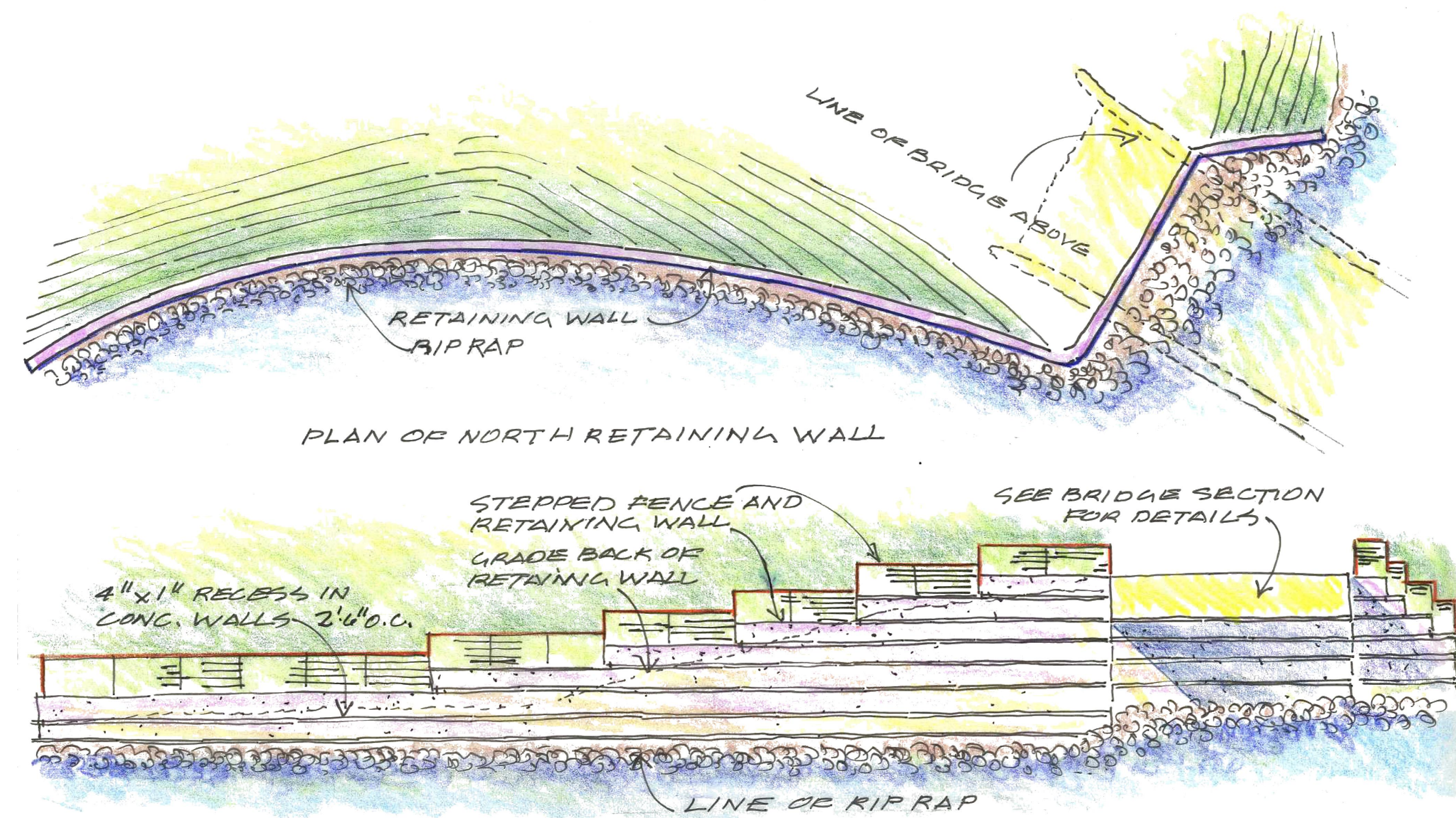
SCHEME ONE ELEVATION OF NORTH RETAINING WALL MEADOW WAY BRIDGE OVER SAN ANSELMO CREEK NOV 11/15
