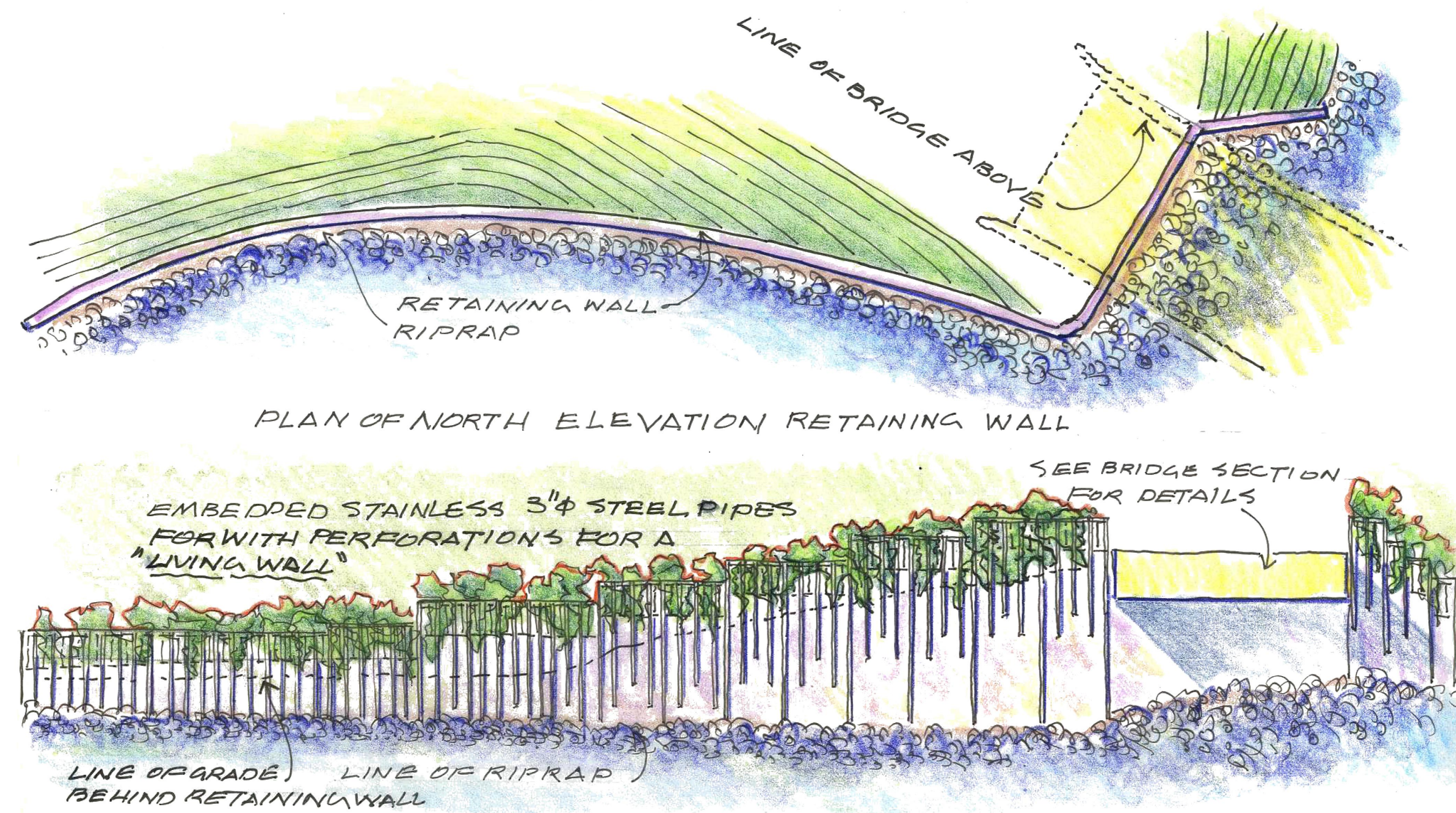
SCHEME TWO ELEVATION OF NORTH RETAINING WALL MEADOW WAY BRIDGE OVER SAN ANSELMO CREEK NOV 10/15
